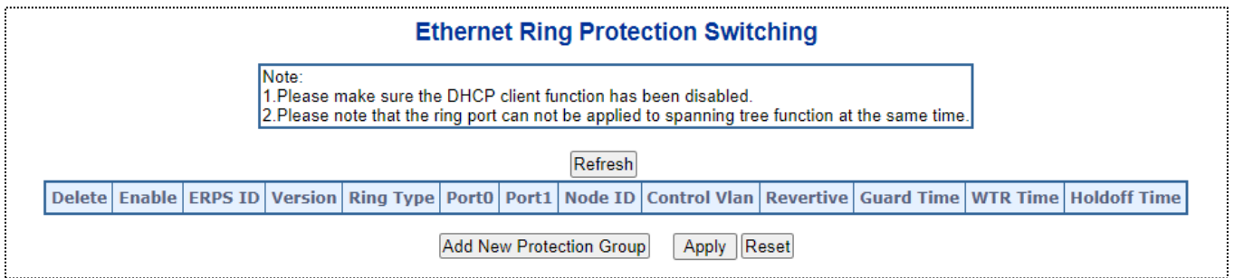
Figure 4-6-1-3: Ethernet Ring Protocol Switch page screenshot
