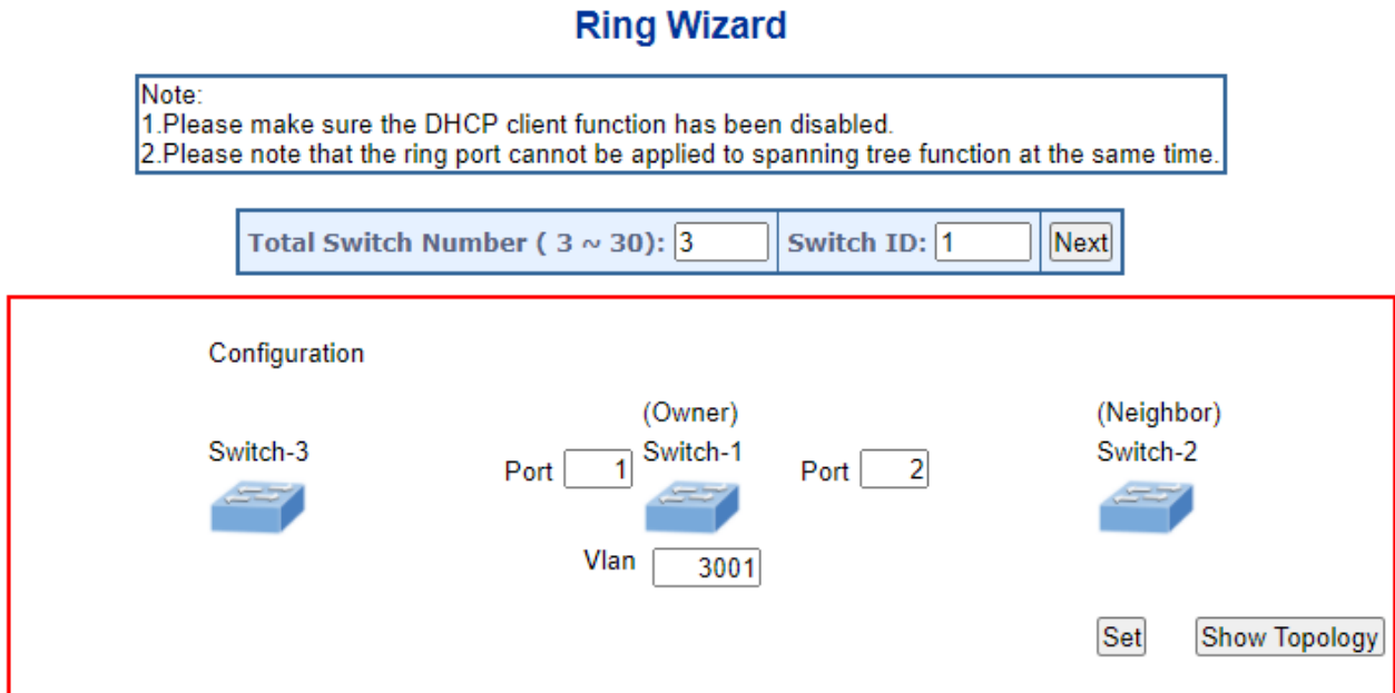
Figure 4-6-1-5: Ring Wizard page screenshot
