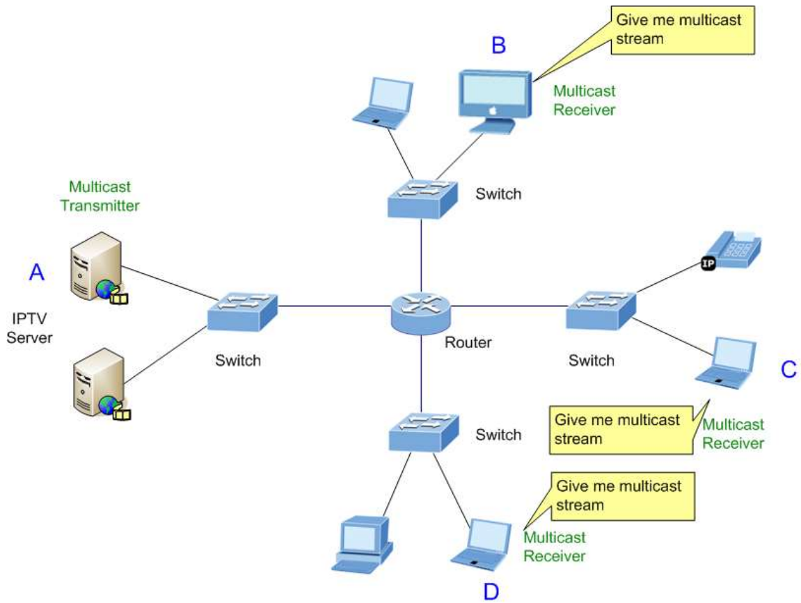
Figure 4-3-78 Multicast Service
