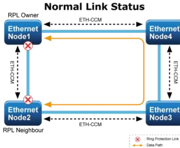
Figure 4-6-1-1 Ring Mode
